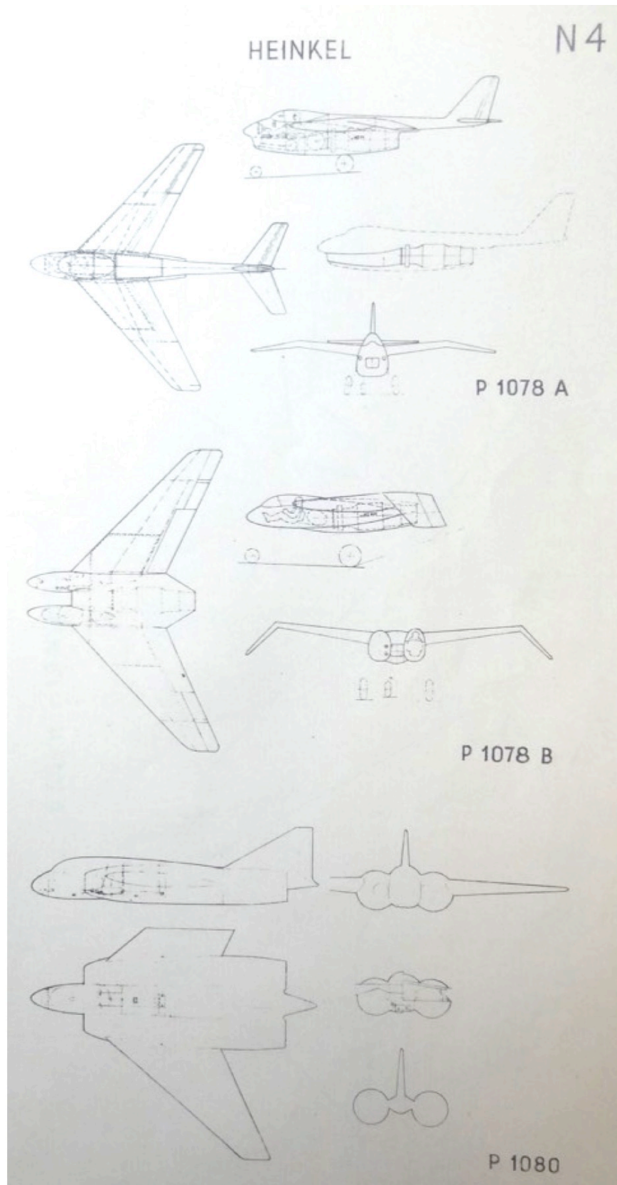
Figure E.22: Wartime Heinkel jet bomber designs now in the U.K. Imperial War Museum, Duxford [Newton 1946].
