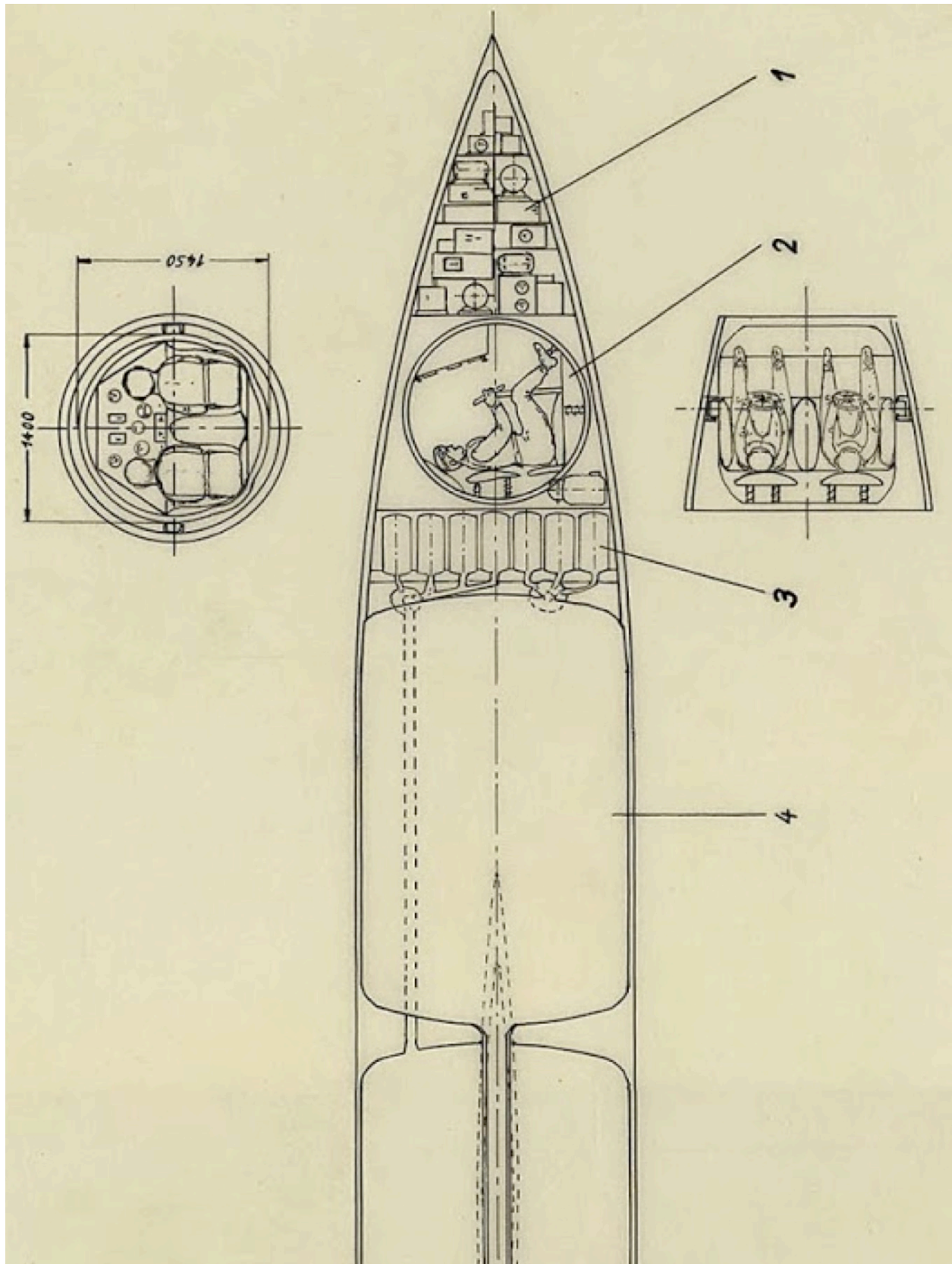
Figure E.112: Detail from Heinz Stoelzel's drawing of the A-9 upper stage showing the two-man crew.
