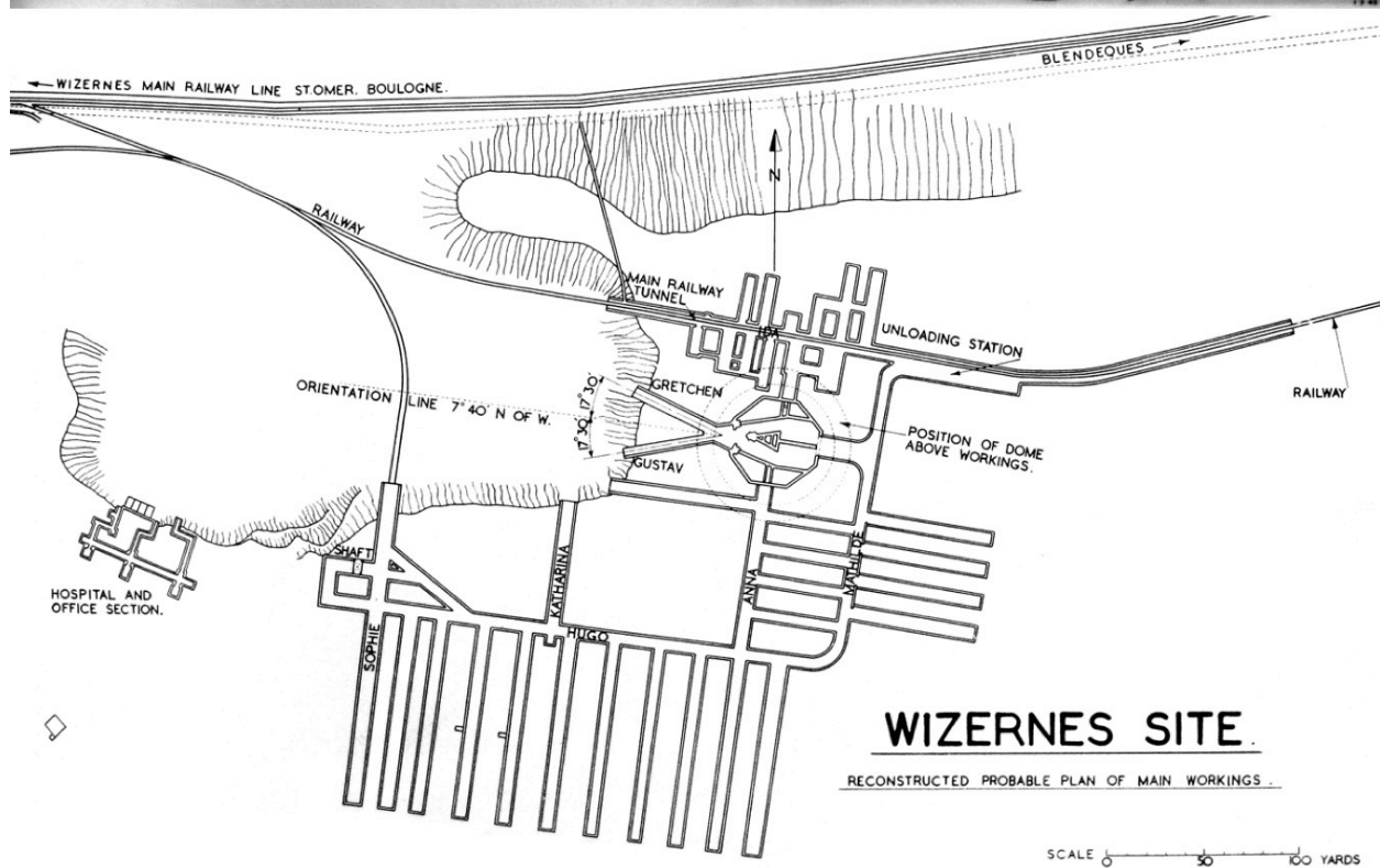
Figure E.60: Layout of the Wizernes underground missile silo/bunker complex on the coast of northern France (built 1943–1944).
