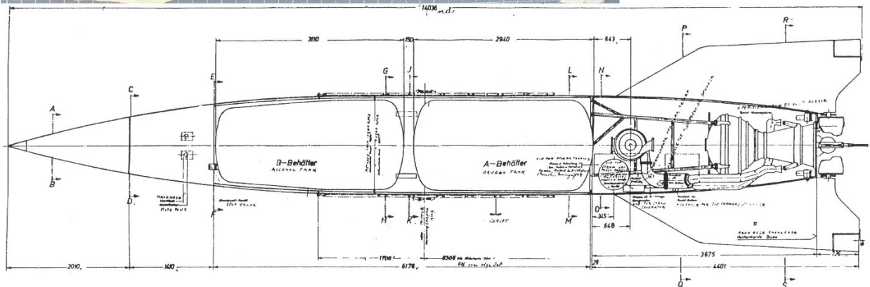
Figure E.51: March 1943 blueprint showing what appears to be a central payload compartment for a modified A-4 rocket [TNA AVIA 40/717, courtesy of Michael Haupt]. It may have been advantageous to carry a heavier-than-initially-planned payload (perhaps the 2-ton Thuringian device [p. 5203]?) closer to the rocket's center of mass instead of in the nosecone. [See Henshall 2000, p. 123.]
