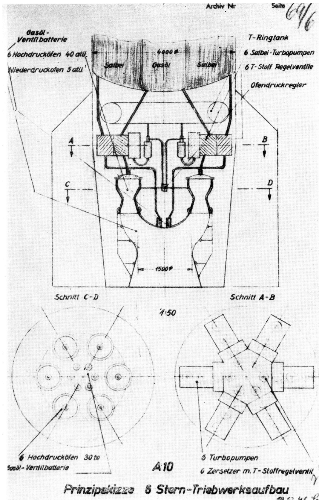
Figure E.37: A-10 rocket engine design using six A-4 engines connected to one large shared exhaust nozzle [Deutsches Museum Archive, photo 32307; Klee and Merk 1963, p. 100].
