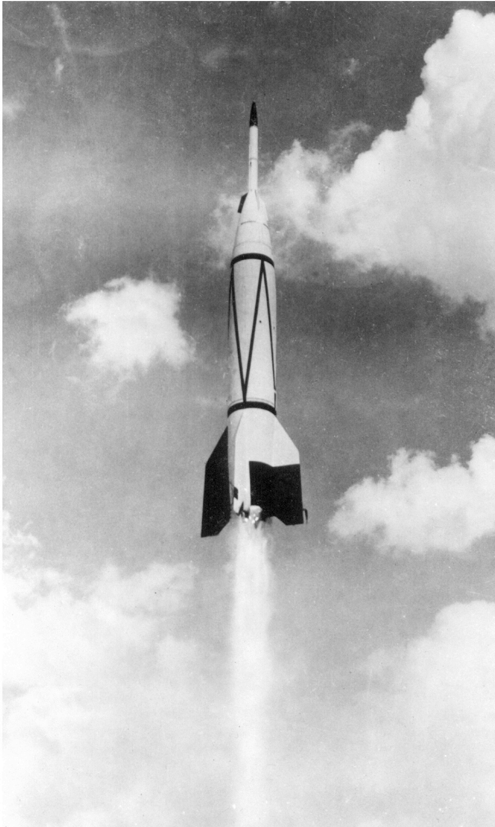
Figure E.77: Bumper 5, an A-4 (V-2) first stage with a small WAC Corporal second stage, was launched in the United States on 24 February 1949 and attained a maximum altitude of 393 km. It may have been based on successful similar wartime German experiments.
