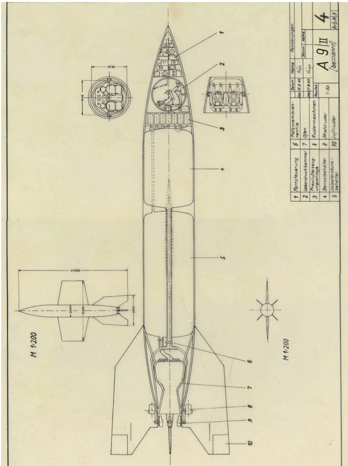
Figure E.111: Design for A-9 upper stage with a two-man crew to be launched into space, hand-copied in 1945 by Heinz Stoelzel. The vast majority of Stoelzel's papers were destroyed after his death, including the A-10 lower stage design if it was in his possession.
