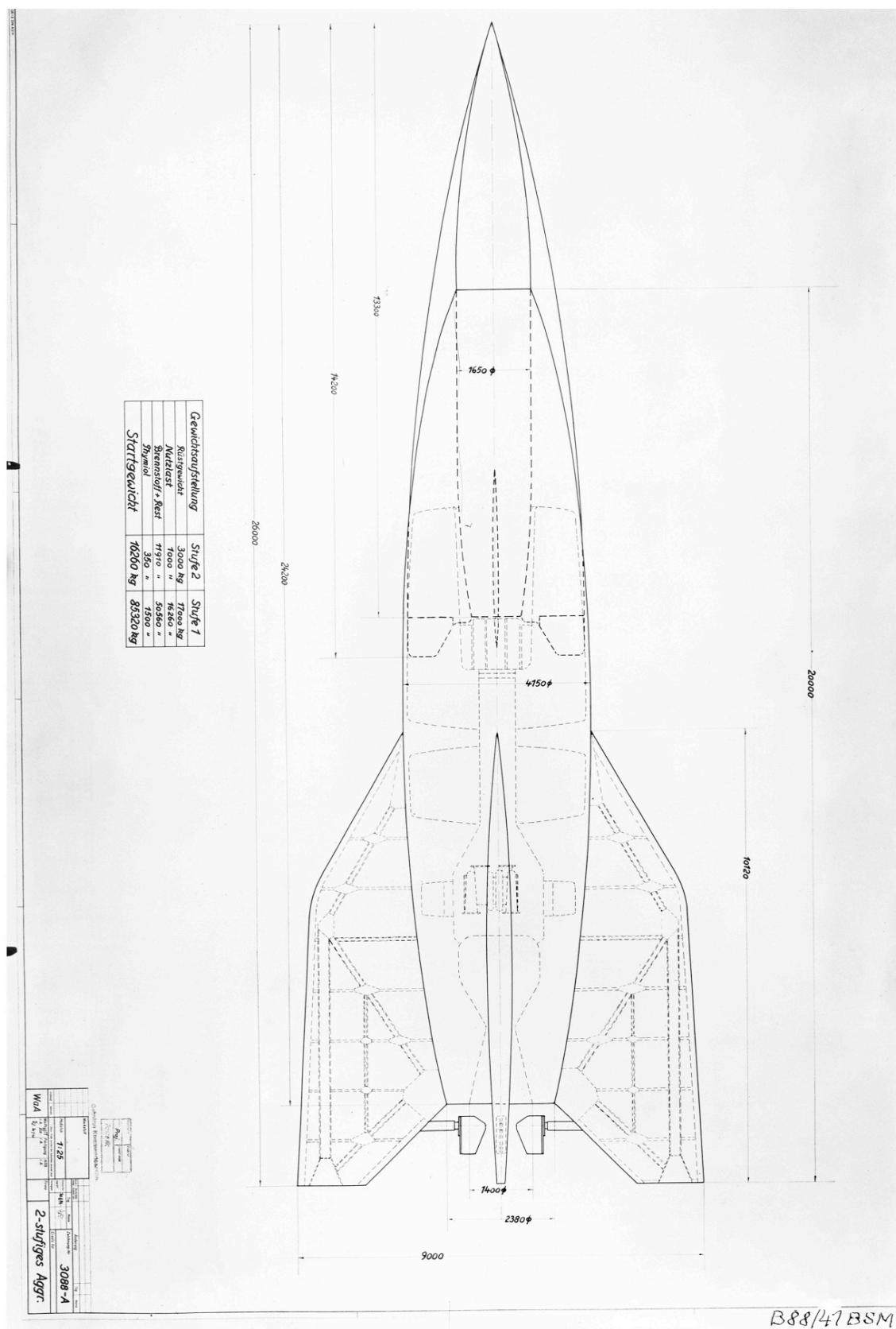
Figure E.36: 1941 design for A-9/A-10 two-stage intercontinental rocket [Deutsches Museum Archive, photo 9664].
