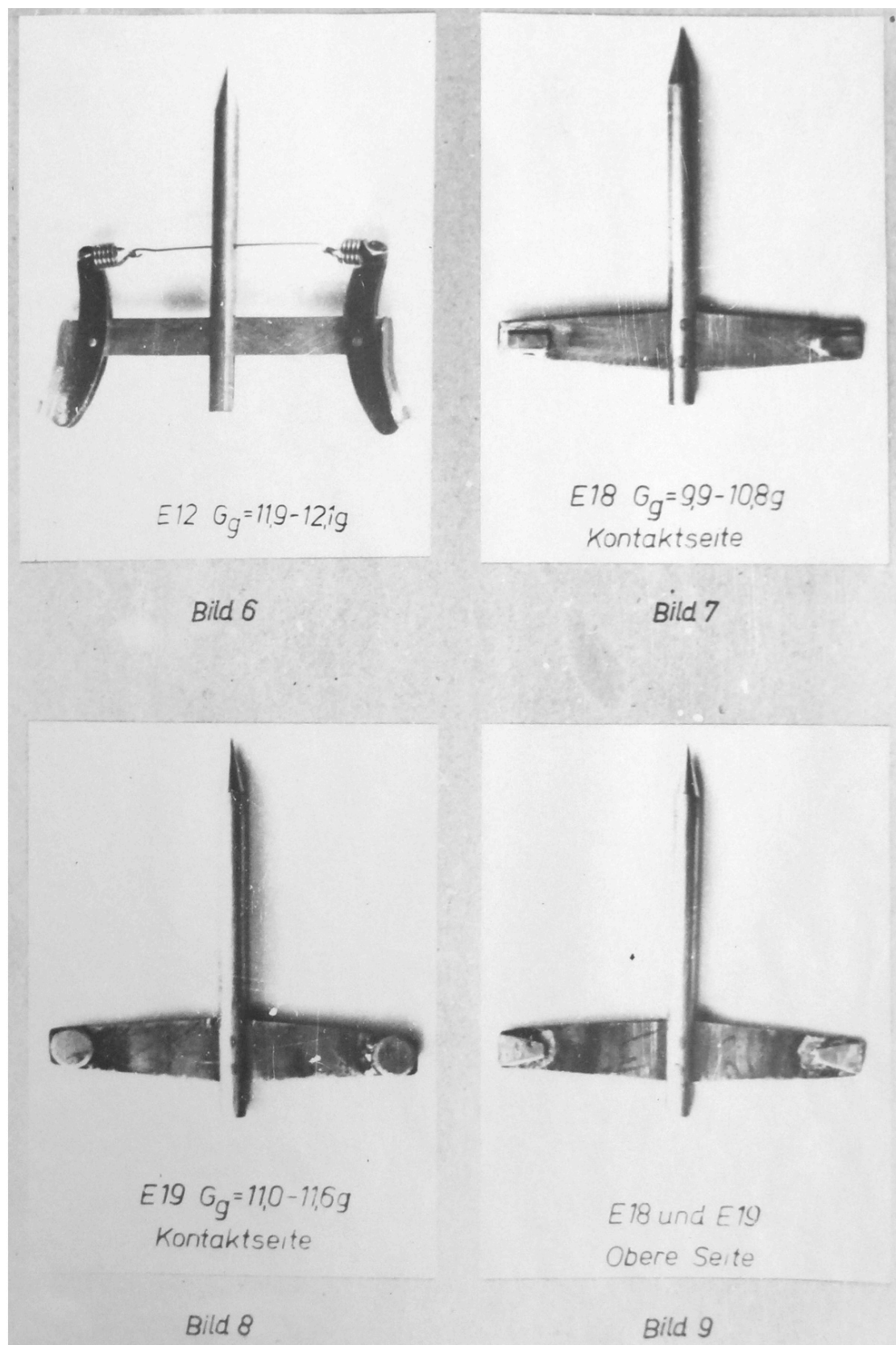
Figure C.155: Part of Joachim Hänsler's 1945 reports on the development and testing of electromagnetic railguns.
