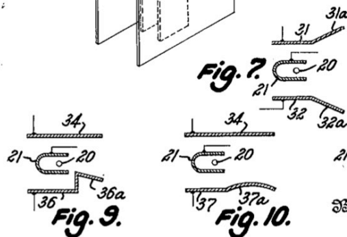
Figure C.12: Figures from one of Rolf Wideröe's wartime patents on particle accelerators.
