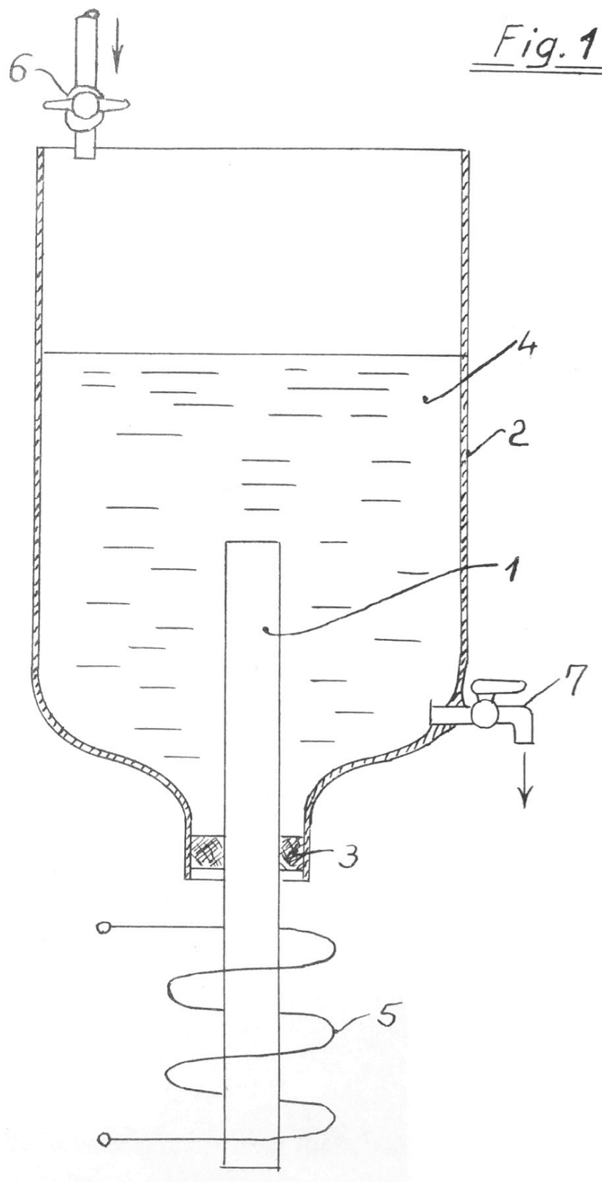
Figure C.112: Ultrasonic sonicator [BIOS 1504].
