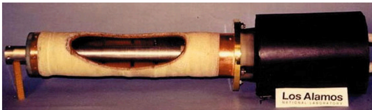
Figure C.65: Example of a modern electromagnetic pulse weapon.
