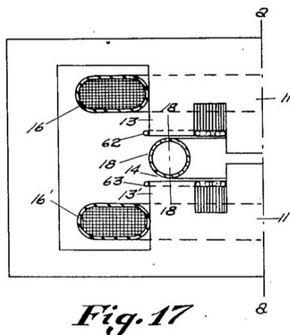
Figure C.6: Figures from one of Rolf Wideröe's wartime patents on particle accelerators.
