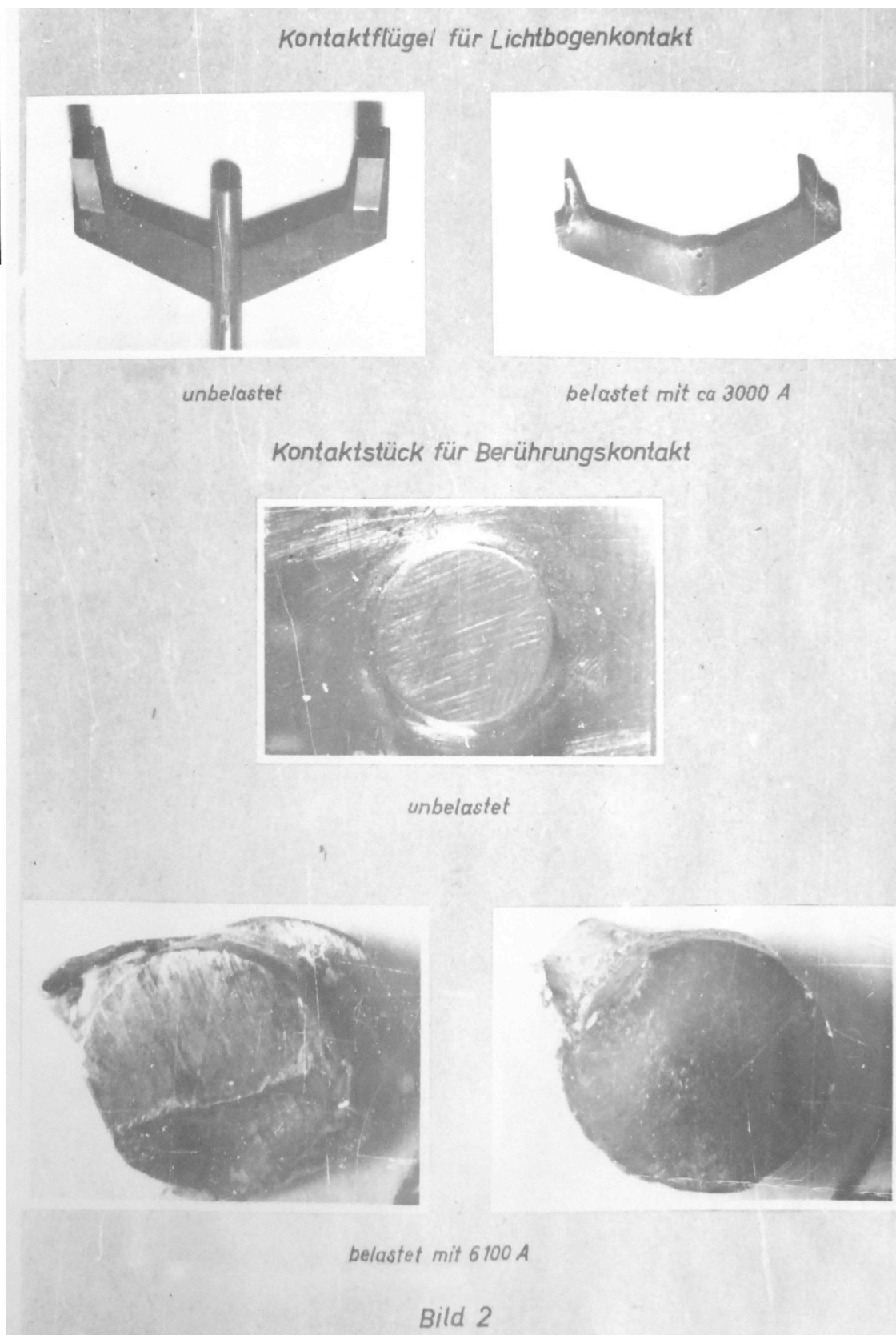
Figure C.150: Part of Joachim Hänsler's 1945 reports on the development and testing of electromagnetic railguns.
