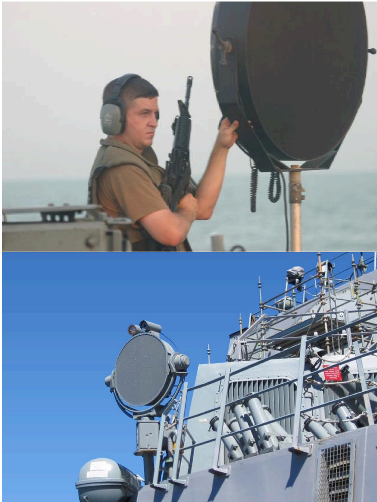
Figure C.124: Modern LRAD (Long Range Acoustic Device) acoustic weapon used by the U.S. Navy and other ships to deter pirates.
