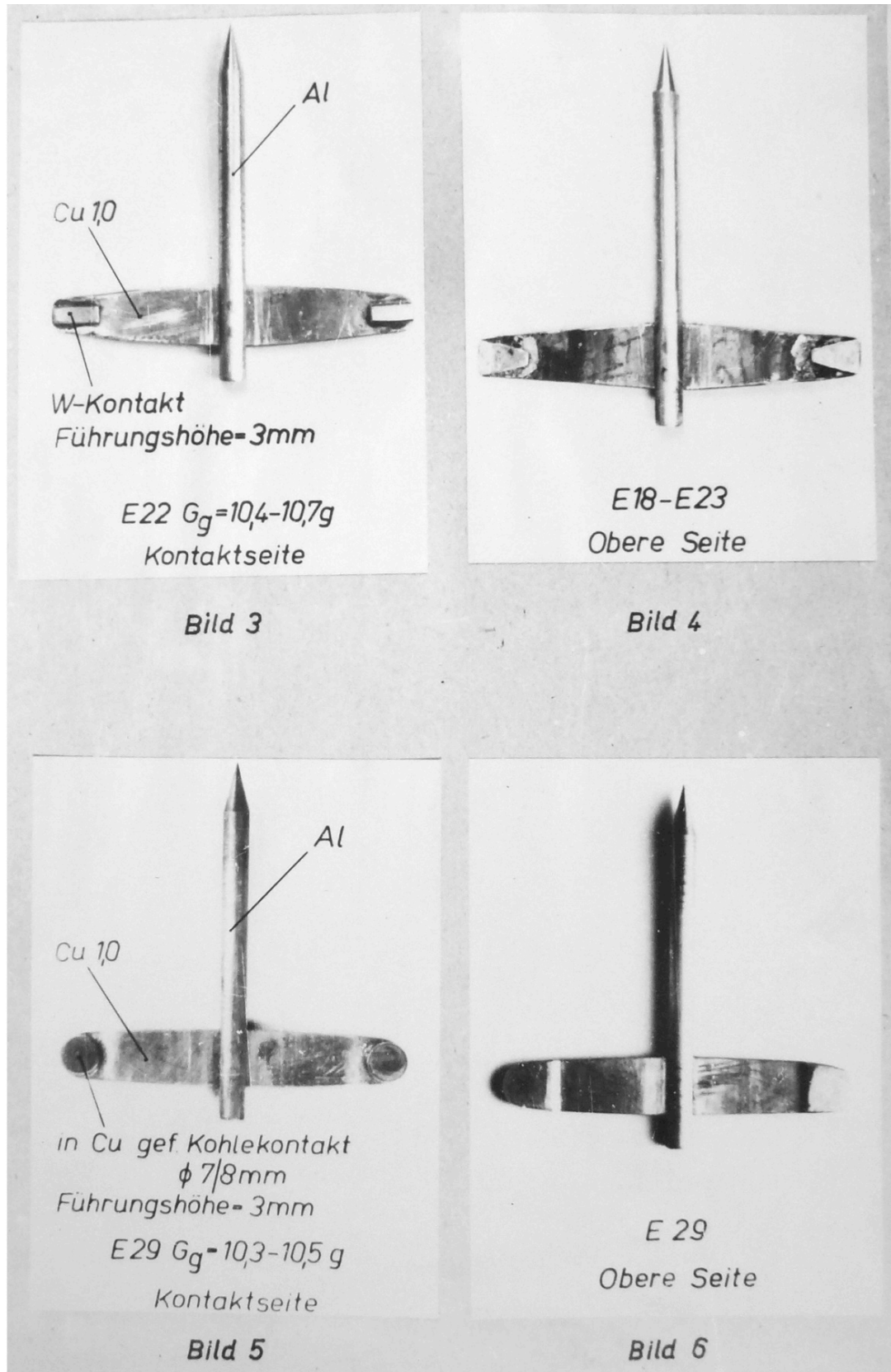
Figure C.159: Part of Joachim Hänsler's 1945 reports on the development and testing of electromagnetic railguns.
