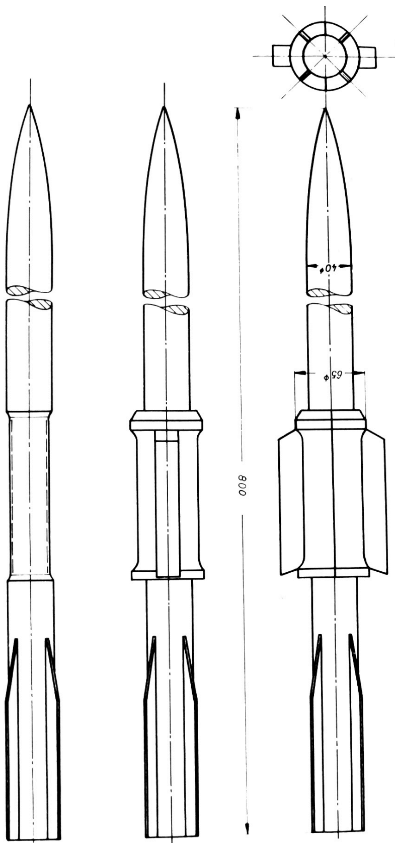
Figure C.144: Part of Joachim Hänsler's 1945 reports on the development and testing of electromagnetic railguns.
