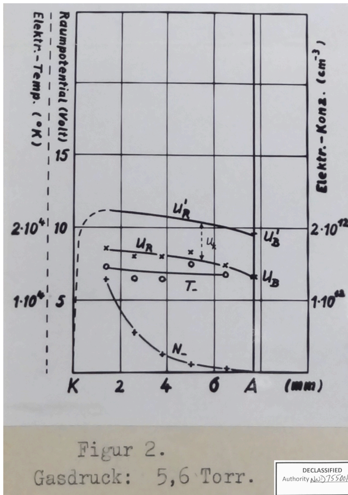
Figure C.95: Wilhelm von Meyeren's 20 February 1945 report on experiments with laser-like monochromatic stimulated light emission from electron population inversions in argon, cesium, or rubidium gases [NARA RG 319, Entry NM3-82A, Box 6, Folder G3].
