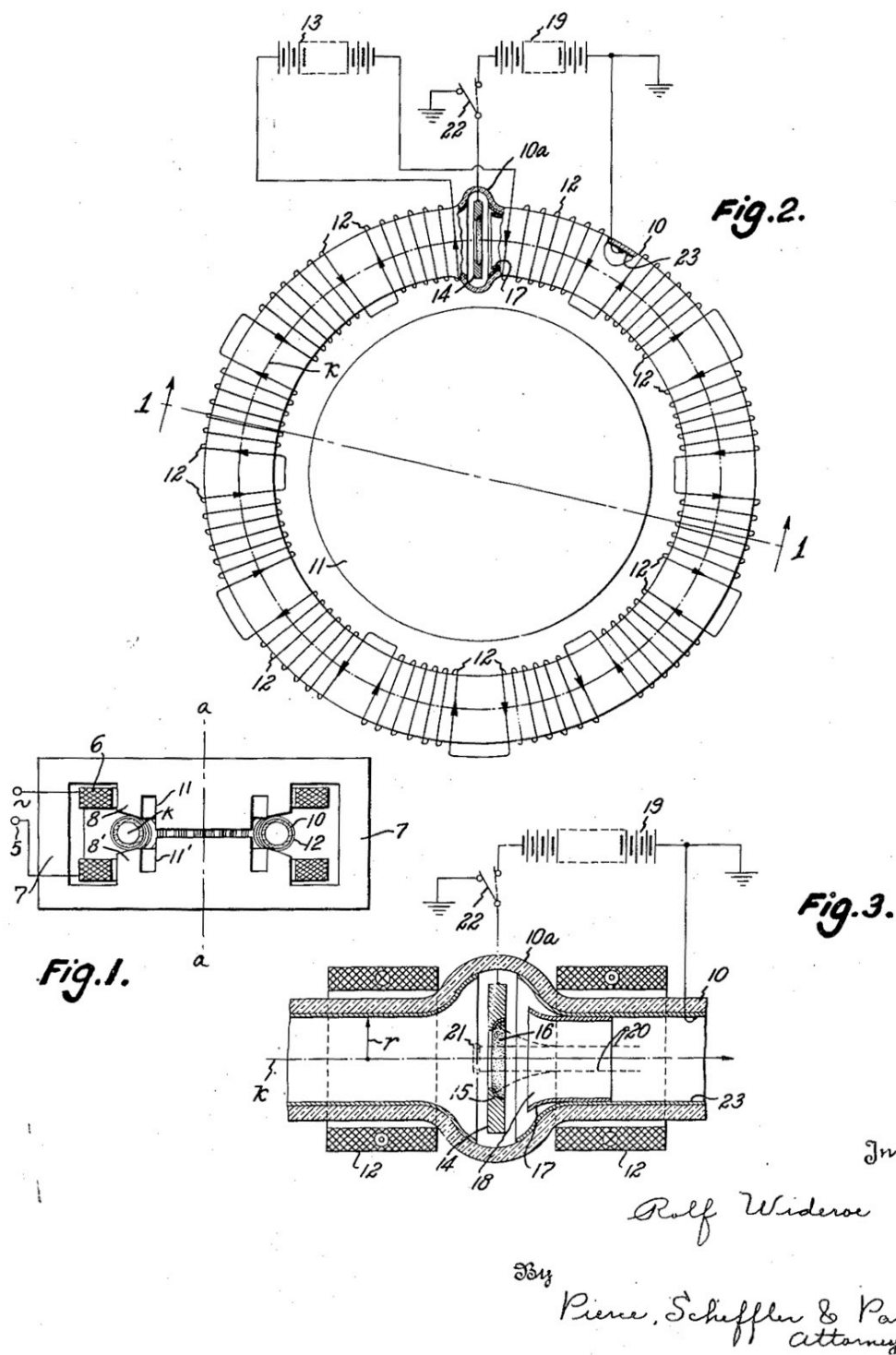
Figure C.11: Figures from one of Rolf Wideröe's wartime patents on particle accelerators.
