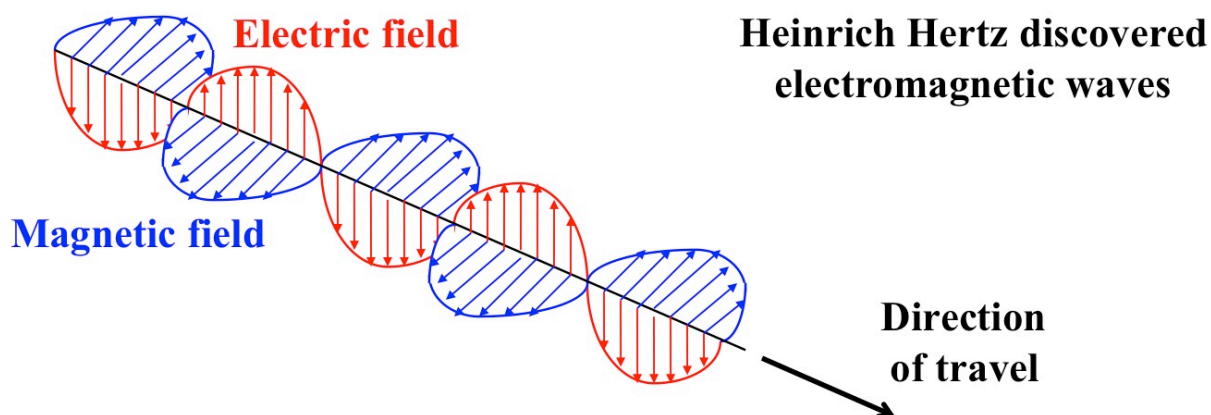
Figure 5.18: Examples of major German-speaking contributions to electromagnetism include Ohm's law for the relationship among voltage, current, and resistance in an electrical circuit; Christian Doppler's explanation for why the frequency and wavelength of waves change when their source is moving; and Heinrich Hertz's demonstration of electromagnetic waves.
