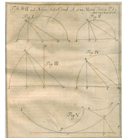
Figure 5.1: Early creators who made significant contributions to applied mathematics and classical mechanics included Christiaan Huygens, Gottfried Leibniz, and Leonhard Euler.
