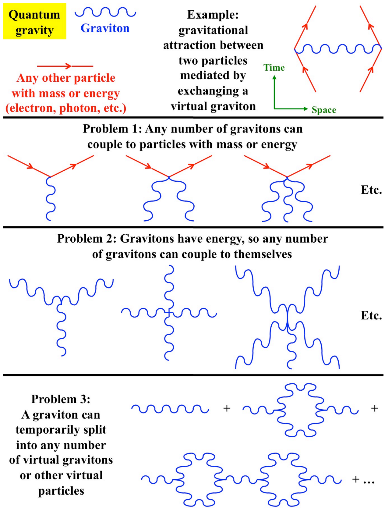
Figure 5.57: Combining special and general relativity with quantum physics yields a theory of quantum gravity, which still suffers from several unresolved mathematical problems.
