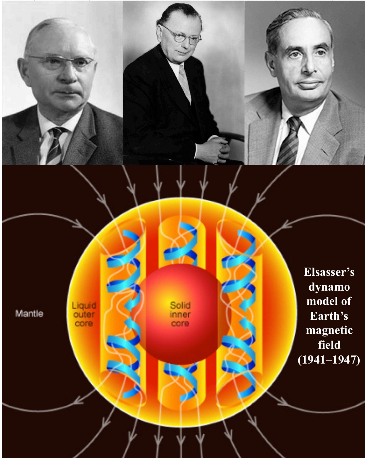
Figure 4.9: Julius Bartels and Gerhard Fanselau made detailed studies of the Earth's magnetic field, and Walter Elsasser developed the dynamo model that explains how the Earth's magnetic field is generated (1941–1947).
