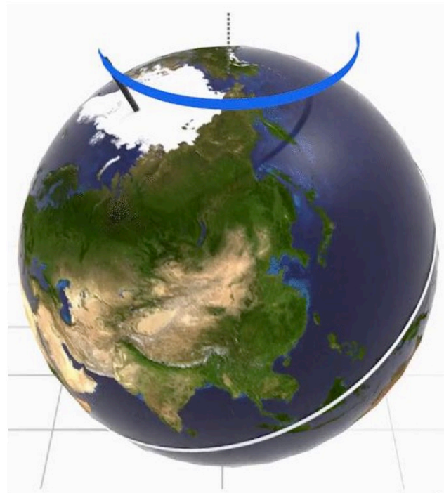
Figure 4.38: Milutin Milanković (or Milankovitch) worked out how periodic changes in the Earth's orbit and axis affect its climate (Milanković or Milankovitch cycles). He also studied similar effects for Mercury, Venus, the Moon, and Mars.
